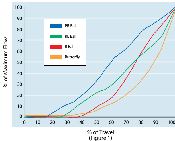
Regulating Valve Flow Curves
